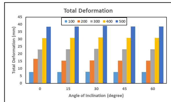
Fig. 6 - Effect of Angle of Inclination on Total Deformation
