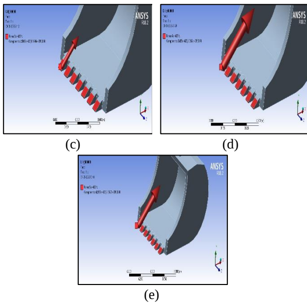
Fig. 3 - Schematic representation of distributed pressure loading applied on the bucket bottom surface and the bucket inclination angles (a) 0^\circ (b) 15^\circ (c) 30^\circ (d) 45^\circ (e) 60^\circ defined with respect to the global X-axis.
