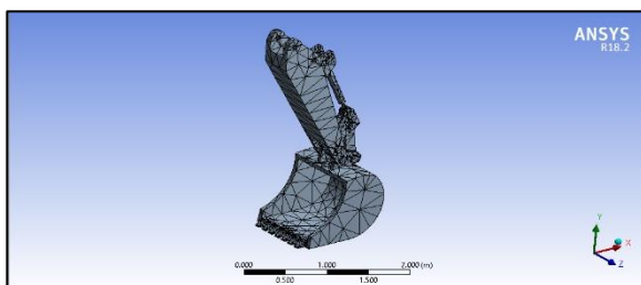
Fig. 4 - Finite element discretization of the excavator arm–bucket assembly showing mesh refinement in critical regions such as the fixed stick end and the bucket–arm joint.
