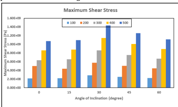
Fig. 7 - Effect of Angle of Inclination on Maximum shear Stress
