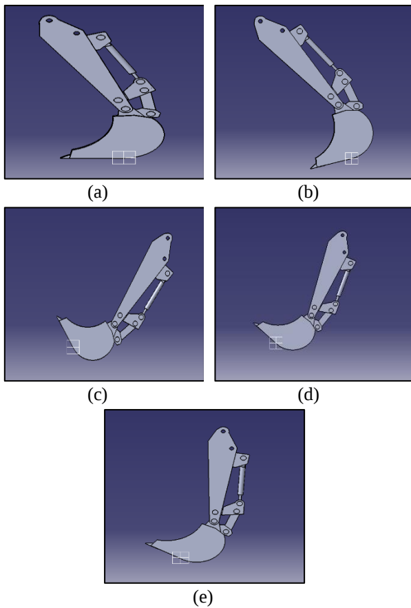
Fig. 1- Three-dimensional geometric model of the excavator arm bucket assembly with inclination angle (a) 0° (b) 15° (c) 30° (d) 45° (e) 60°
